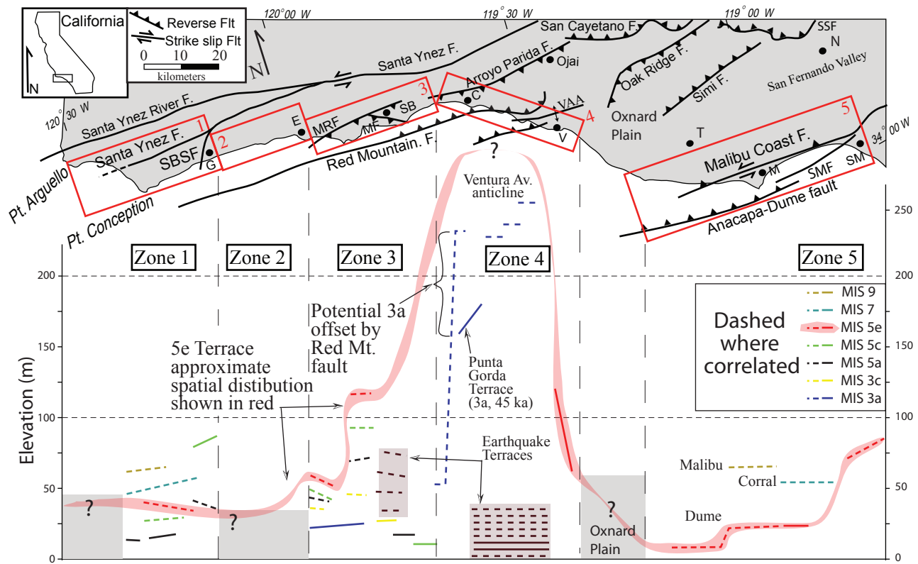
Figure 2. Longitudinal cross-section showing the Santa Monica Mountains and interpreted terraces in elevation. Note, these elevations are correlated to absolute ages: MIS 9; Mission Ridge, Carpinteria, Avenue Anticline, Ventura, V; T; Northridge, Santa Monica.
